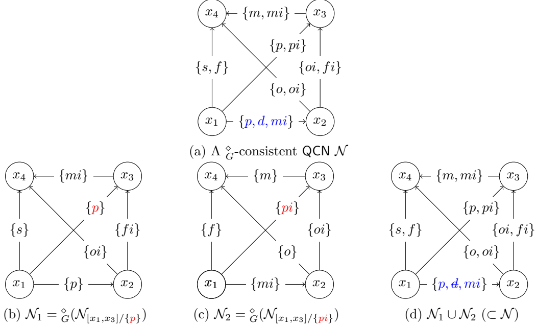
Figure 2: A \diamond_G -consistent QCN of Interval Algebra along with a demonstration of how enforcing \blacklozenge_G^U -consistency can further eliminate invalid atoms; G is the complete graph on \{x_1, x_2, x_3, x_4\}
