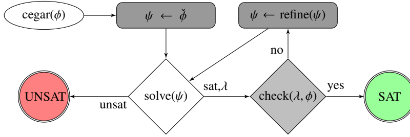
Fig. 2. The CEGAR framework with under-approximation
