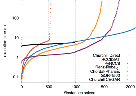
Fig. 6. Runtime distribution on the second set
