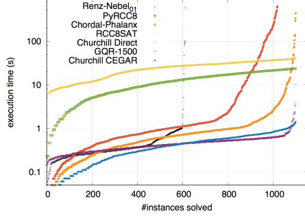
Fig. 5. Runtime distribution on the first set
